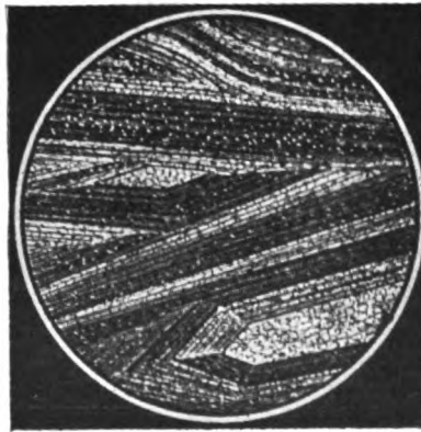
Fig. 2—Magnified surface of manganese bronze after being slightly scratched by grit. Magnified 48 diameters
